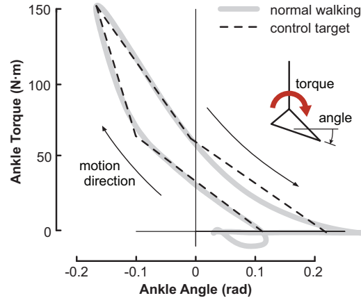
Figure 2.2: Impedance control law used during walking trials. Desired torque is a piecewise linear function of ankle position, with separate dorsiflexion (negative velocity) and plantarflexion (positive velocity) phases. Default curve parameters were selected to roughly match the torque-angle relationship observed for the biological ankle during normal walking. Plantarflexion segments were manipulated across conditions to alter the net positive ankle joint work over the step cycle.
