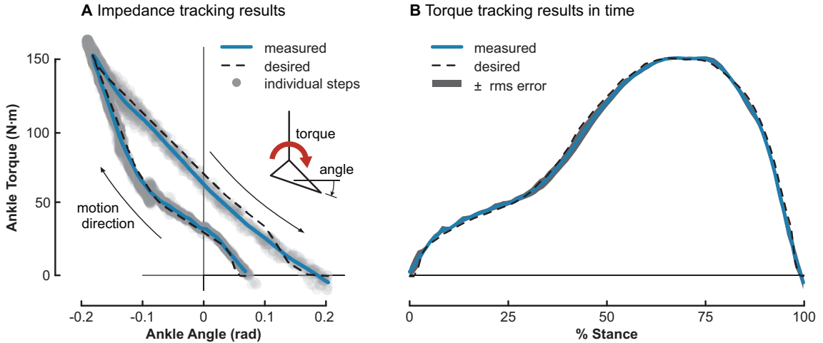
Figure 2.4: Tracking of impedance control law during walking. A Measured torque-angle relationship as one subject with unilateral transtibial amputation walked at 1.25 \text{ m}\cdot\text{s}^{-1} for one minute (52 strides). Each step resulted in a similar amount of net joint work, 7.88 \pm 1.28 \text{ J} , visible here as work loop area. B Joint torque over the stance period during one minute of walking, normalized to % stance. Average stance duration was 0.58 \pm 0.02 \text{ s} . The average RMS torque error was 2.8 \text{ N}\cdot\text{m} . Note that time-trajectory error appears smaller than error in angle-torque space, while the latter is more meaningful in terms of work production or absorption.
