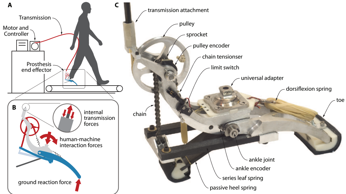
Figure 2.1: Mechatronic design of the universal prosthesis emulator. A The system comprises three elements: (1) powerful off-board motor and control hardware, (2) a flexible tether transmitting mechanical power and sensor signals, and (3) a lightweight instrumented end-effector. This division of components was chosen to maximize responsiveness and minimize end-effector mass during treadmill walking. B Free-body diagram of the end effector. Internal Bowden cable transmission forces pull the synthetic rope upwards while equally and oppositely pushing the aluminum frame downwards. Rope tension is transmitted through the pulley, sprocket, chain, and leaf spring, giving rise to a ground reaction force at the toe. The effect is equivalent to an ankle plantarflexion torque, resulting in a reaction force and moment at the interface with the human user. C Photograph of the instrumented prosthesis. A pulley-sprocket component magnifies transmission forces and allows direct measurement of spring deflection. A tensioning spring keeps the chain engaged. A limit switch protects against excessive plantarflexion. A universal adapter attaches to the socket or prosthesis simulator worn by the user. A dorsiflexion spring comprised of rubber bands retracts the toe, e.g., during leg swing. Fiberglass leaf springs provide series elasticity for ankle torque measurement and control. A separate leaf spring directly connected to the frame (not the toe) comprises the heel.
